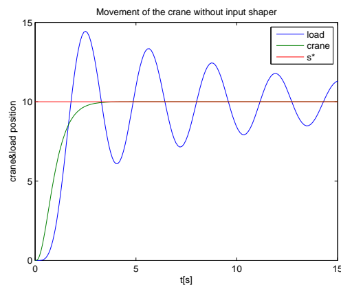
Fig. 6. Movement of the crane without ZV-filter.
