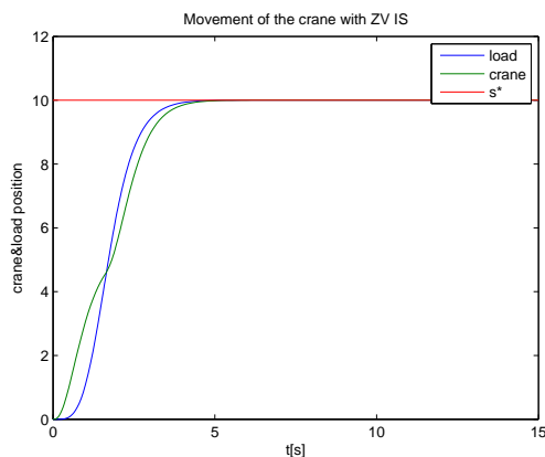
Fig. 8. Movement of the crane with ZV-filter.
