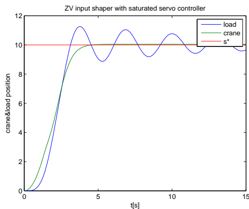
Fig. 9. Movement of the crane with ZV-filter and saturated servo controller.
